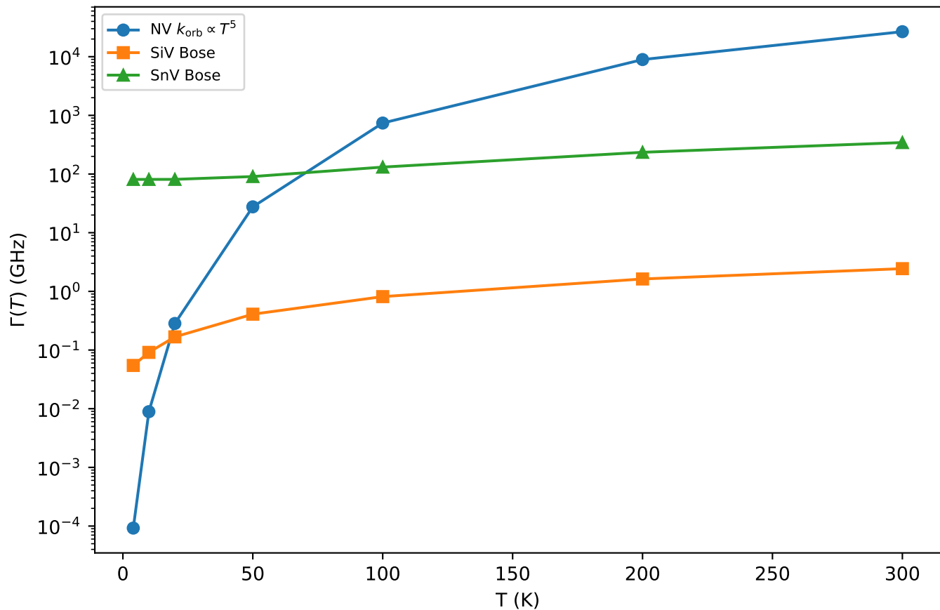
Finite- T rate mapping (NV spans \sim 8.5 decades, group-IV narrow)
